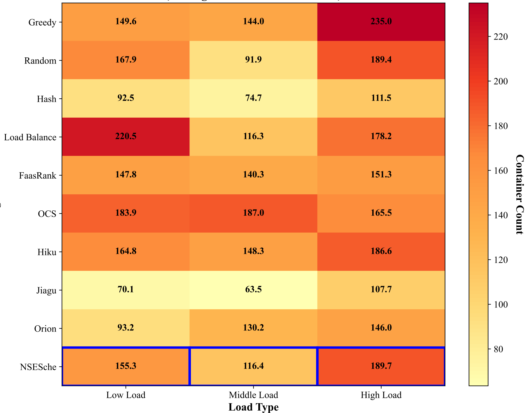
Container Count Heatmap (Average Number of Containers)
